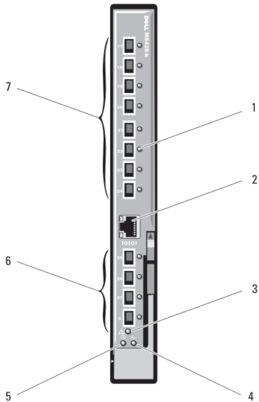
Abbildung 24. 10-Gbit-Converged-Network-Switch Dell PowerConnect M8428-k
